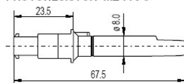
PHOTORESISTOR MZ 770 S
