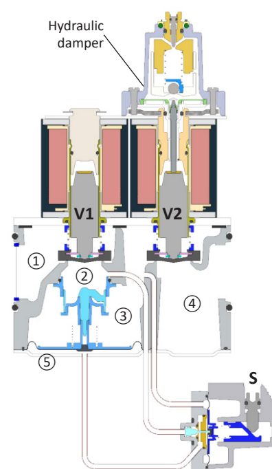
Sectional drawing of multifunctional gas valve M3C**S
